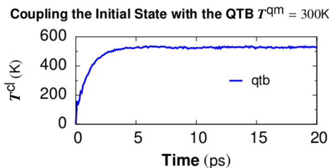
Figure 1. Classical temperature T_{cl} = \sum \frac{mv_i^2}{3Nk_B} vs. time for coupling the \alpha -quartz initial state with the quantum thermal bath at target quantum temperature T^{qm} = 300K . The NpH ensemble is used for time integration while QTB provides the colored random force. T^{cl} converges at the timescale of damp which is set to be 1 ps.
